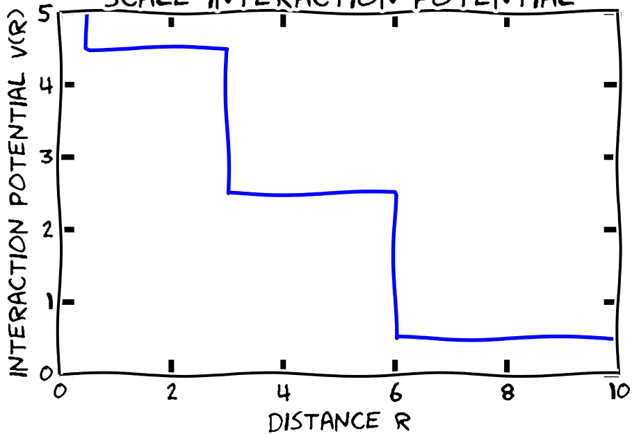
REPULSIVE DISCRETE STEP MULTI-SCALE INTERACTION POTENTIAL
