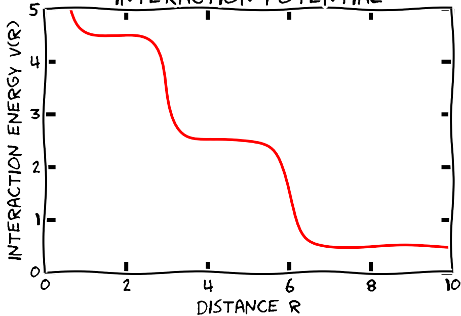
REPULSIVE SMOOTH MULTI-SCALE INTERACTION POTENTIAL
